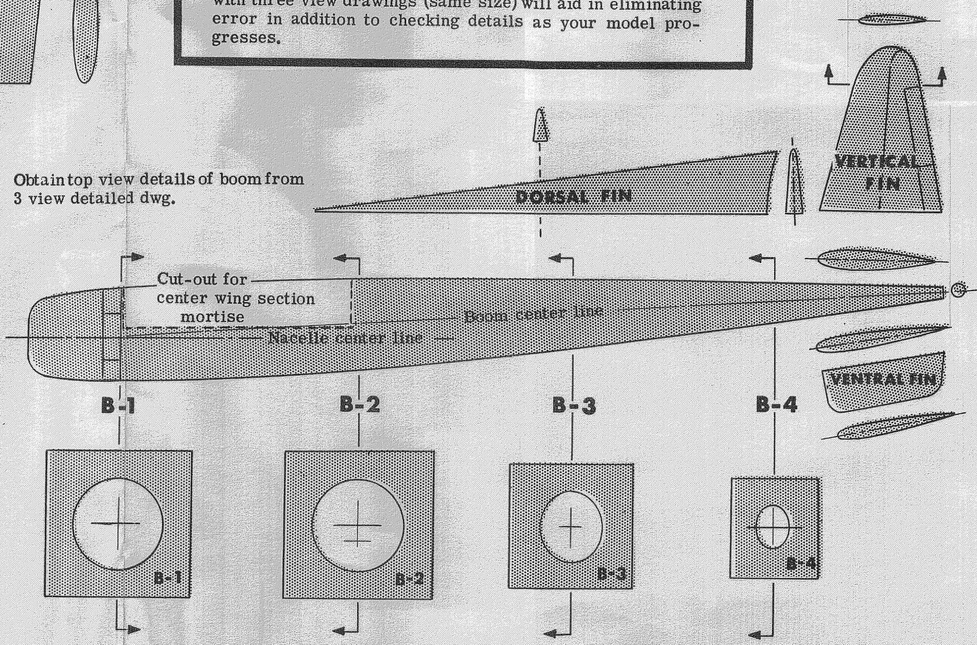
NACELLE-BOOM EMPENNAGE SECTION [ 2 Required ]
